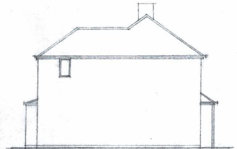
NORTH ELEVATION AS EXISTING 1:100
